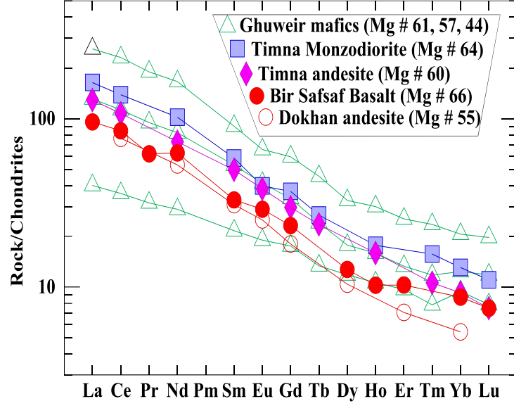
Figure 3. Chondrite-normalized Patterns for the Ghuweir Mafics and the Equivalent Rocks from the Adjacent Countries. The Mg #s are Calculated According to the Formula Mg \# = \frac{\text{mol. prop. Mg}}{\text{mol. prop. Mg} + \text{mol. prop. Fe}} \times 100 .
